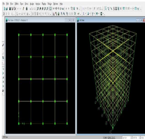
Geometry of Symmetrical Building without Shear Wall.
