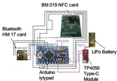
Fig.1. Construction scheme
